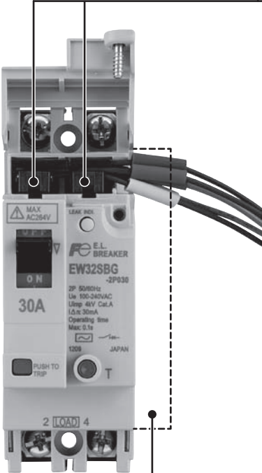
2-pole product
