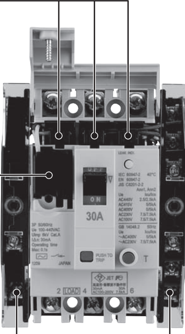
3-pole product
